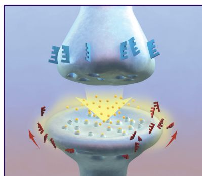
CB1 receptor
